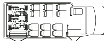
12 Passengers and 2 W/C
