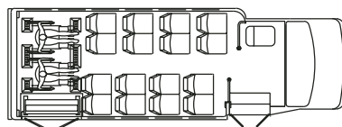
16 Passengers and 2 W/C
