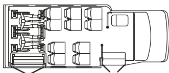
10 Passengers and 2 W/C
